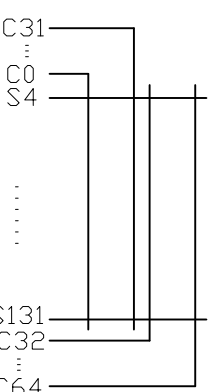
Panel wiring Details
