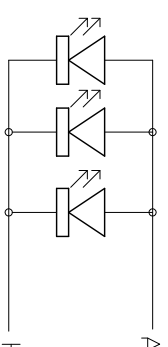
Backlight Circuit
